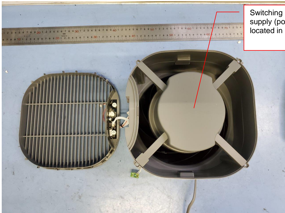
PCB Box
