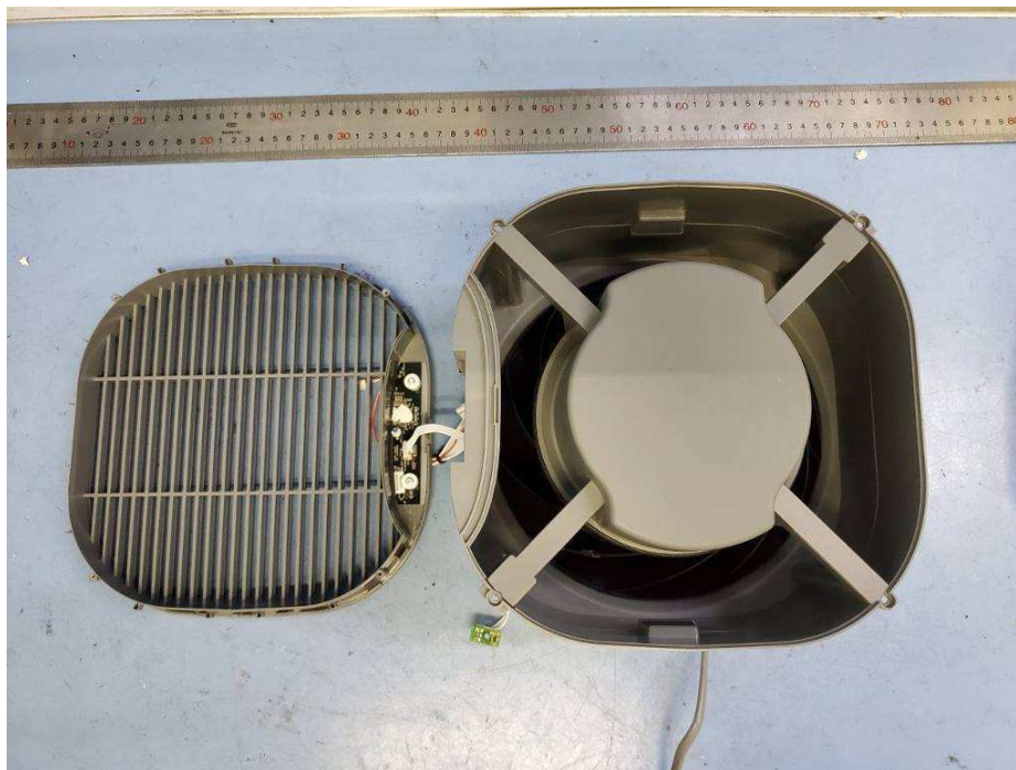
PCB Box
