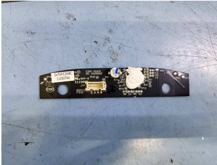
control PCB
