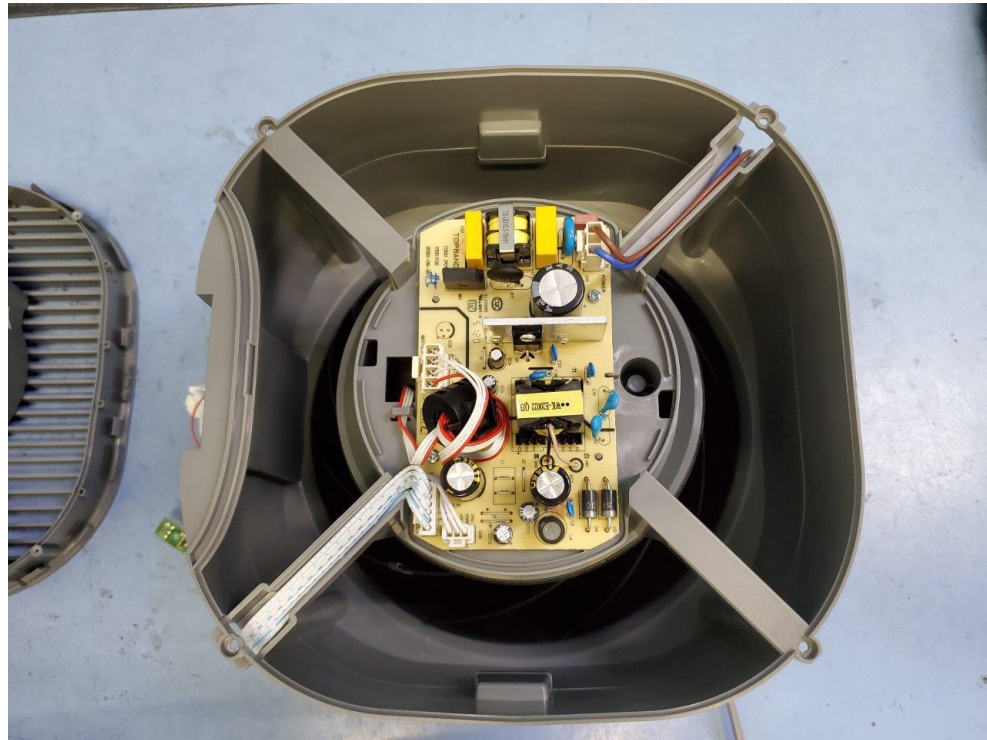
Front view of Power PCB
