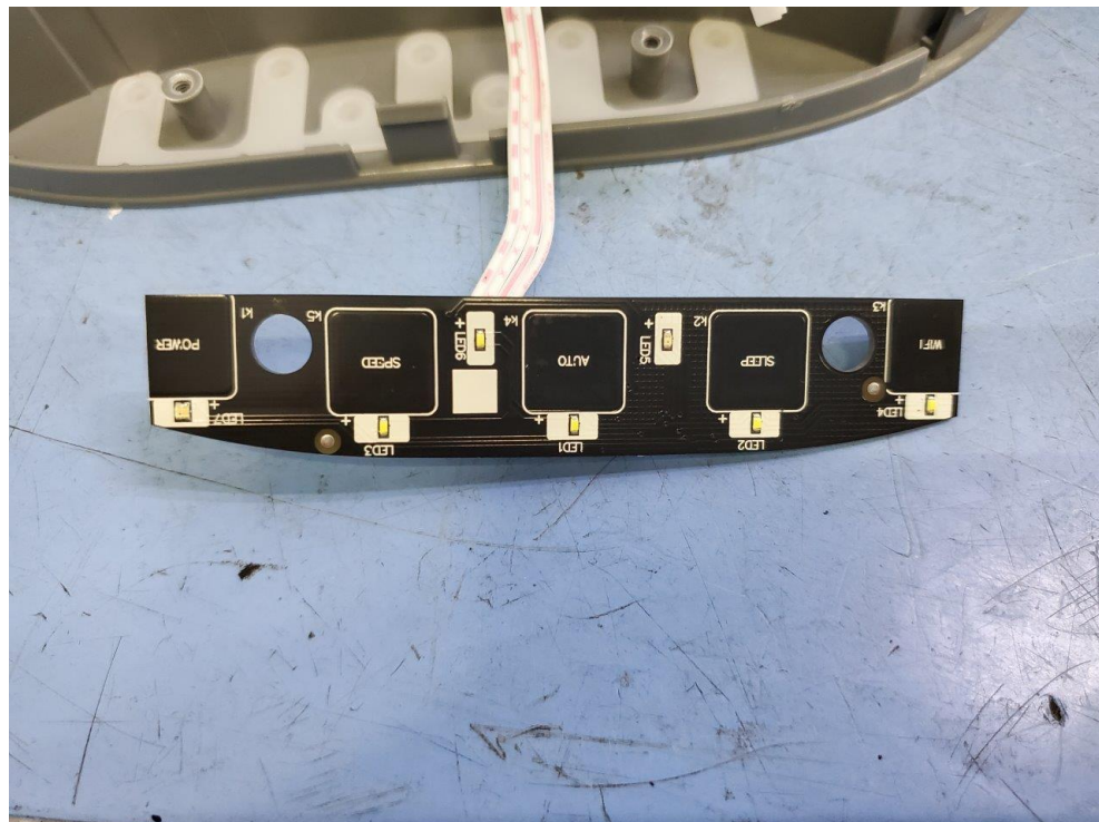
Front view of Control PCB
