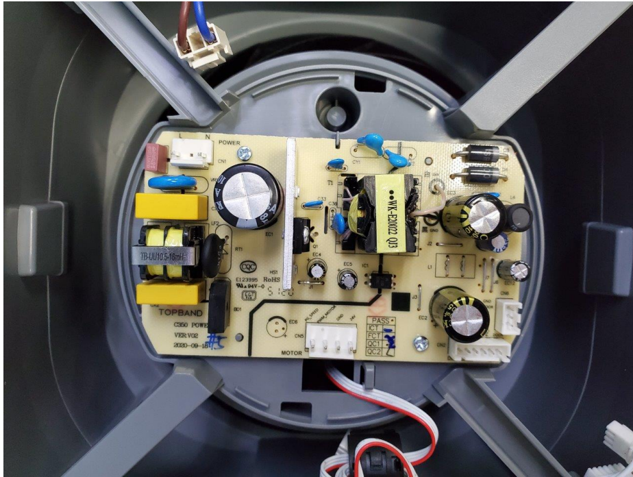
Top view for power PCB (Switching power supply)
