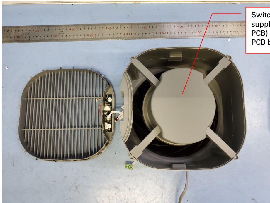
Internal view (remove top cover)
