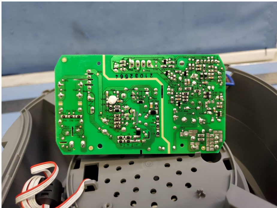
Bottom view of Power PCB (Switching power supply)
